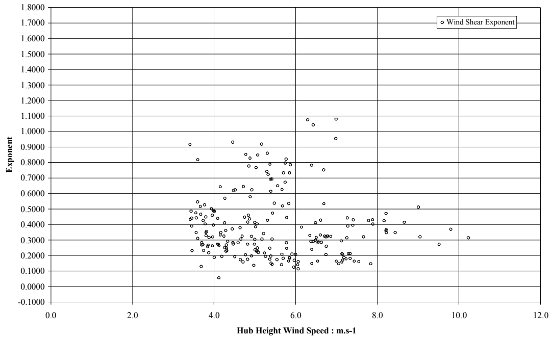
Steadings Wind Farm: October (Partial Data) Wind Shear Exponent
