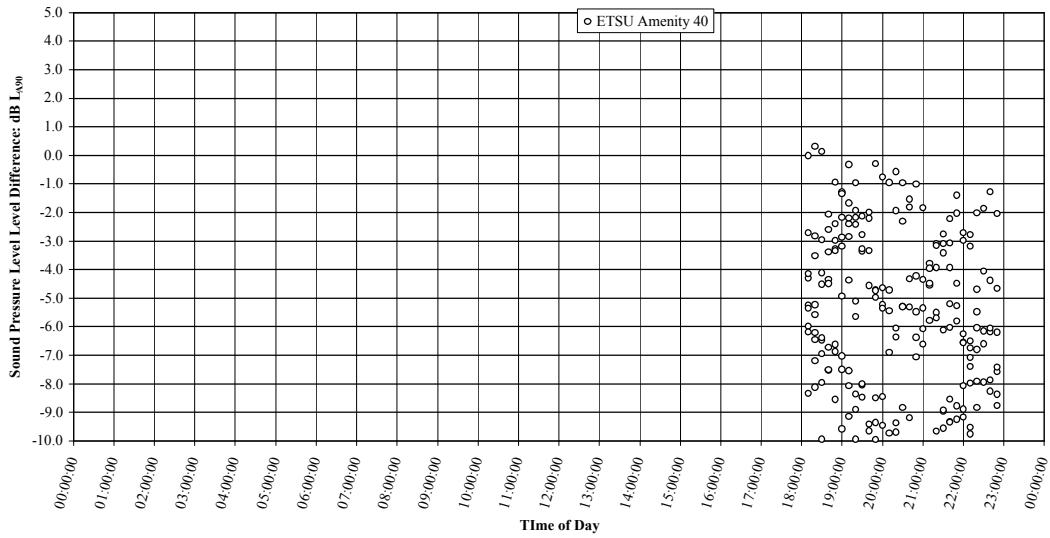
Great Bavington: October (partial data set) ETSU-R-97 Compliance: The greater of 40 dB L A90 or Background + 5 dB Hard Ground: Warranted SWL Amenity Hours
